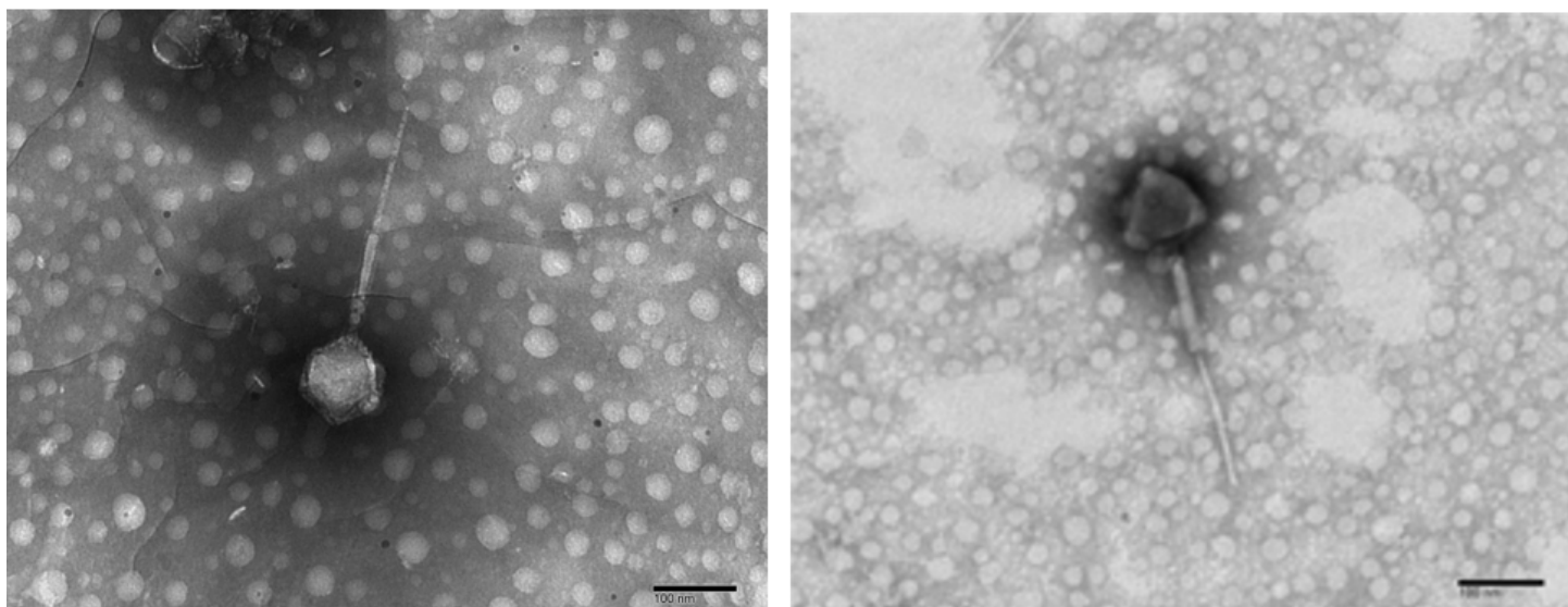
Figure 4. Transmission Electron Micrograph of bacteriophage KP-2 capable of infecting different genotypes of ESBL-producing K. pneumonia .
